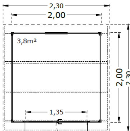
Grundriss / floor plan
